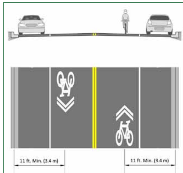
Figure 7.13. Sharrow (shared lane marking). Situation shown here maintains parking on both sides of the street. Source: AASHTO 2010
