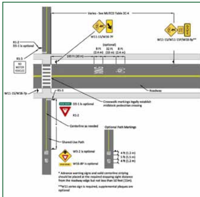
Figure 7.3. Intersection Conditions for Midblock Trail/Road Intersections: Yield and Stop Controlled
