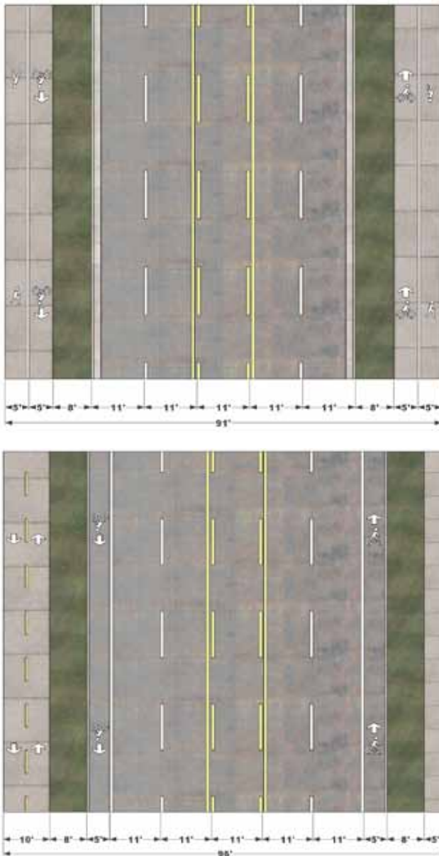
Figure 7.12. (continued) Five-lane sections: Top, one-way sidepaths without bike lanes; above, two-way sidepath with bike lanes
