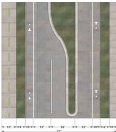
Figure 7.9. (left) Two-lane divided section with sidepath
