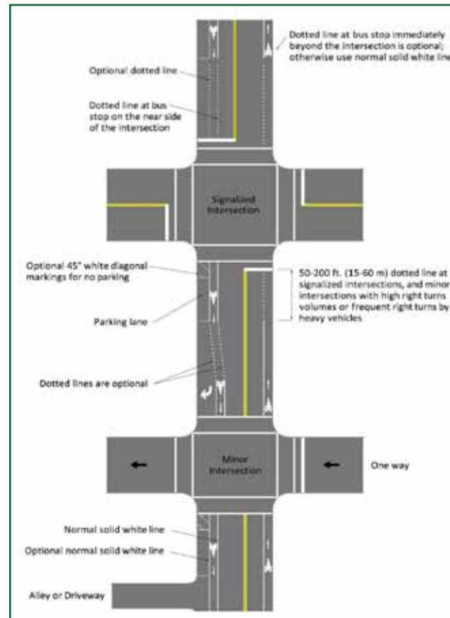
Figure 7.7. Bike Lane Pavement Markings. Source: AASHTO 2010
