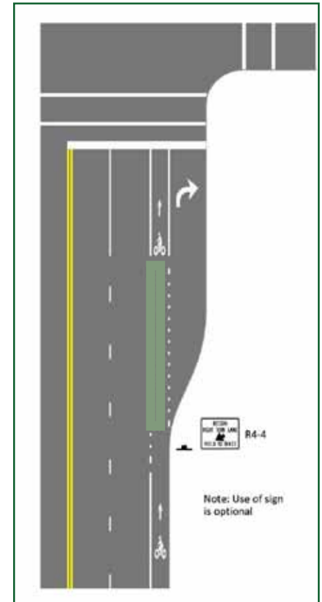
Figure 7.8. Bike Lane Pavement Markings at RTO Lane. Right-turning traffic crosses the direct bicycle lane to the right turn only lane. This condition may arise at major street intersections in the intra-urban system. Source: AASHTO 2010
