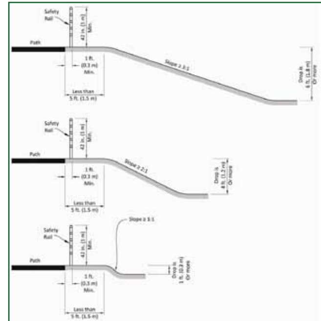
Figure 7.2. Railings and Trail Separations from Adjacent Steep Slopes
