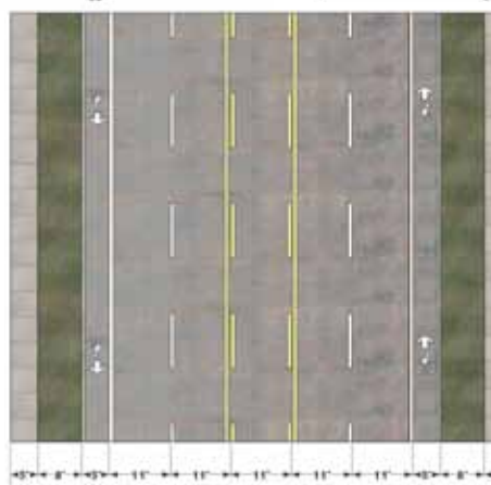
Figure 7.11. (left) Four-lane divided section with sidepath
